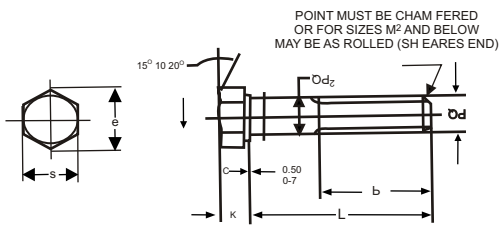
HEX BOLT
