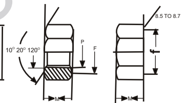
HEX NUT / LOCK NUT
