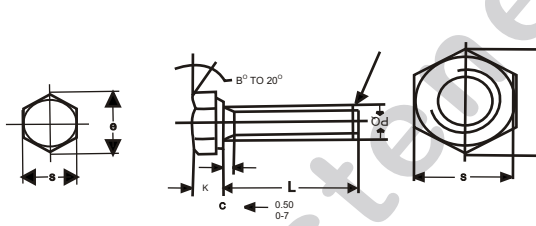
HEX SCREW
